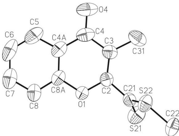
Figure 3 ORTEP view of the X-ray diffraction structure of 74 with atom numbering. Thermal ellipsoids are drawn at the 50% probability level. Hydrogen atoms are not shown.
