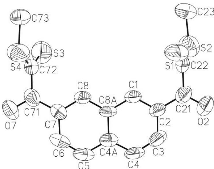
Figure 2 ORTEP view of the X-ray diffraction structure of 71 with atom numbering. Thermal ellipsoids are drawn at the 50% probability level. Hydrogen atoms are not shown.
