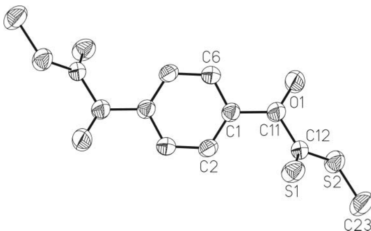
Figure 1 ORTEP view of the X-ray diffraction structure of 7 . Since the molecule exhibits a center of symmetry, the numbering is given for only one half of the atoms. Thermal ellipsoids are drawn at the 50% probability level. Hydrogen atoms are not shown.
